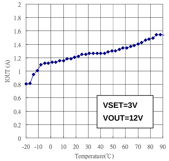
OVER CURRENT TRIGGER POINT V.S. TEMPERATURE
