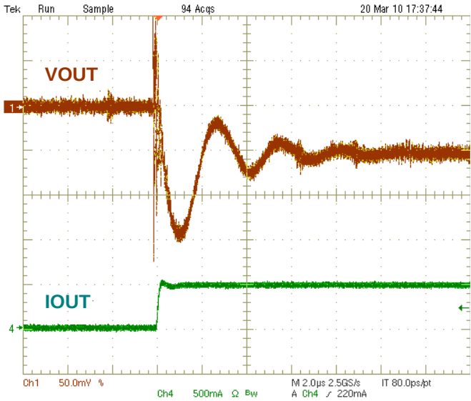
LOAD TRANSIENT
