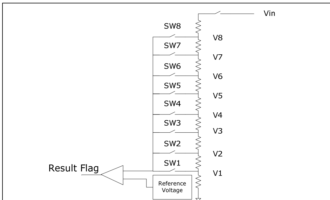
Fig. 7 Architecture of Voltage Detector
