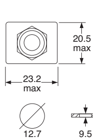
'PO' Actuator and body - push button function (8500 only)
