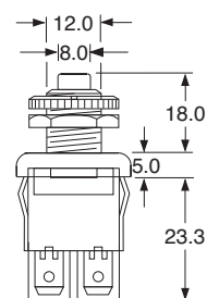
'PO' Actuator and body - push button function (8500 only)
