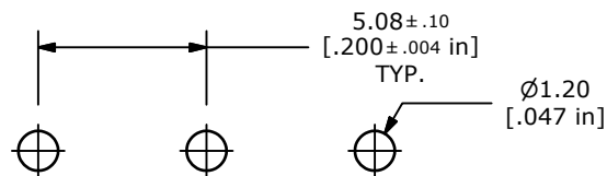
P.C. MOUNTING
