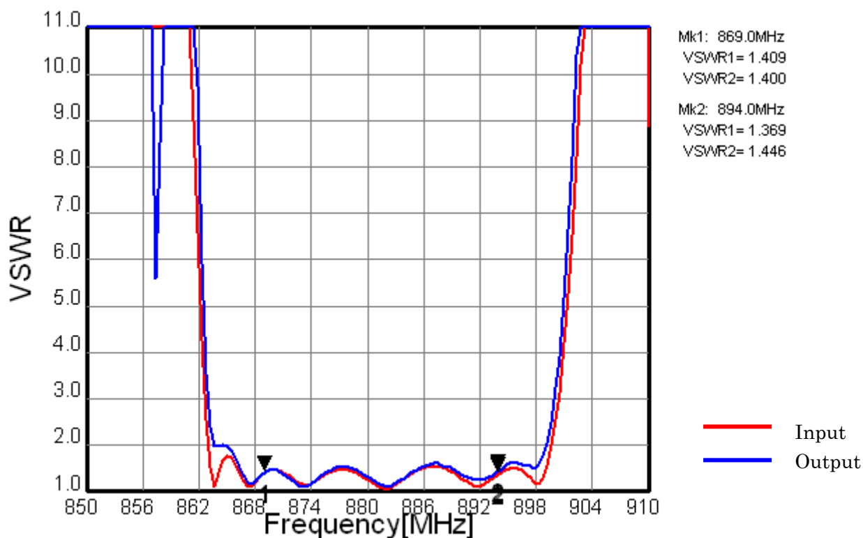
Fig.2 VSWR
