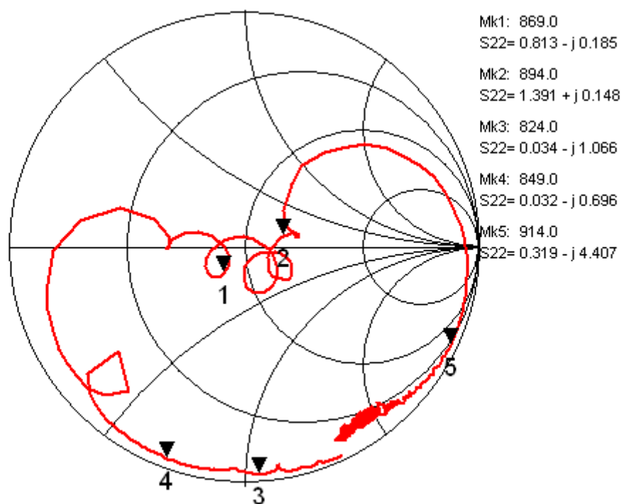
Fig.6 Output Impedance (Balance)
