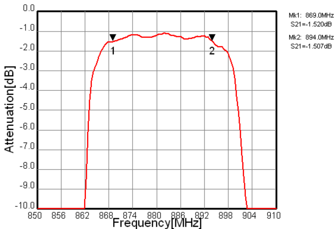
Fig.3 In-band Characteristics
