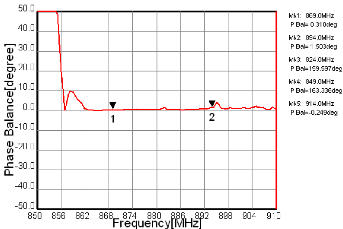
Fig.8 Phase Balance
