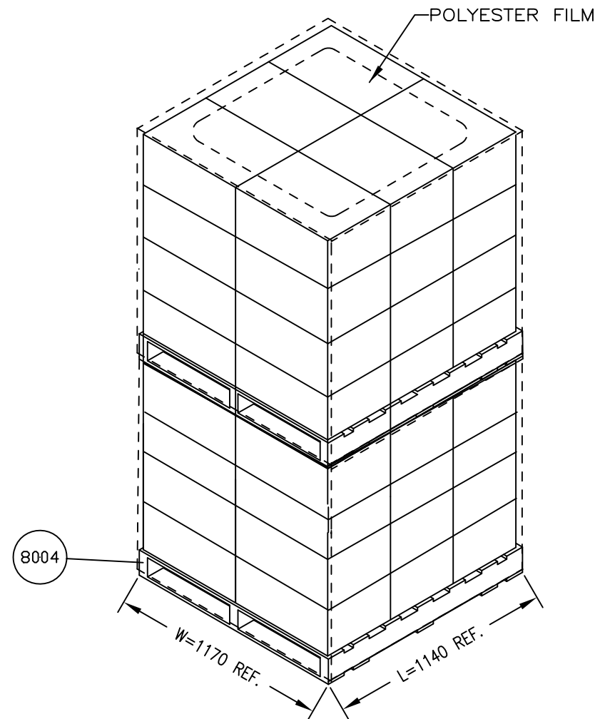
PALLET ASS'Y DRAWING:
