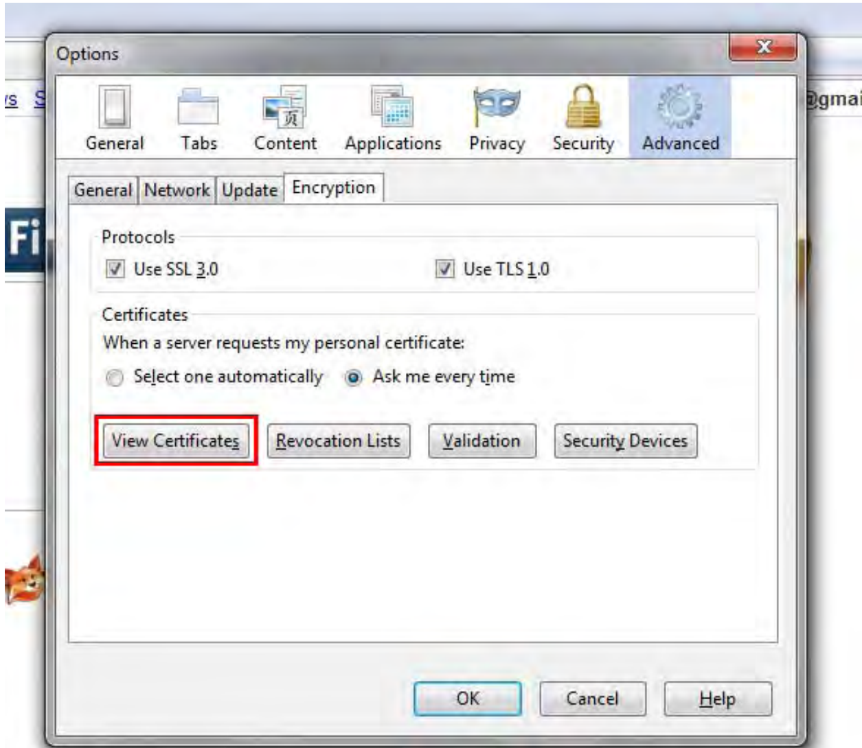
Figure 58: View Certificates
