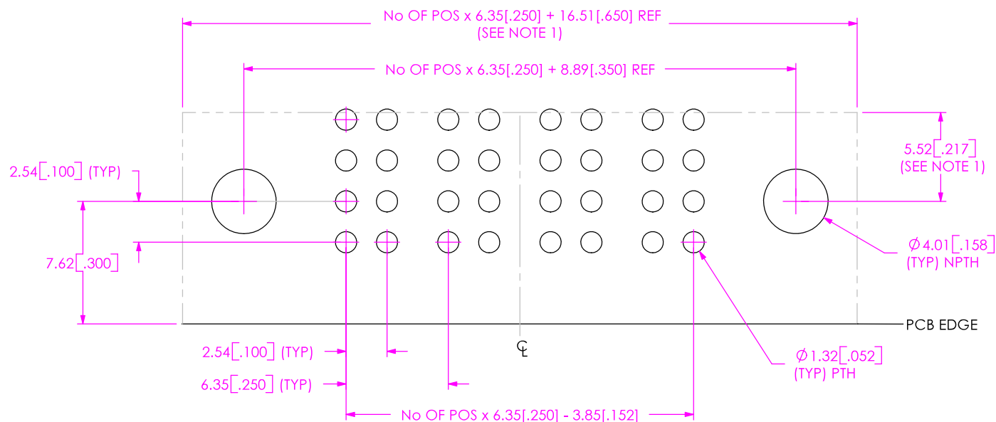
FIG. 1 PCB LAYOUT FOR PET-XX-XX-XX-RA-SD SHOWN
