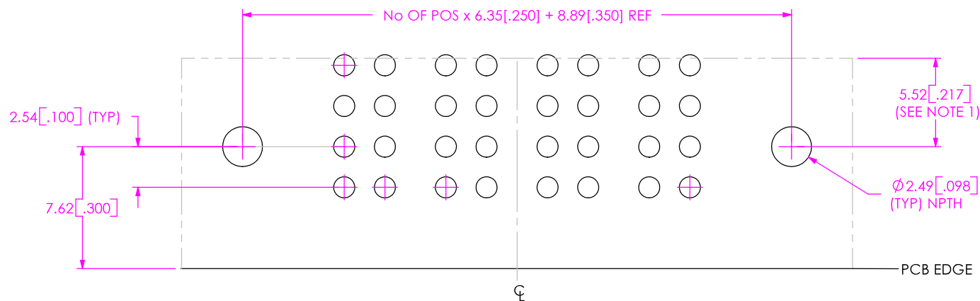
FIG. 2 PCB LAYOUT FOR PET-XX-XX-XX-RA-LC SHOWN (SAME AS FIG. 1, UNLESS OTHERWISE STATED)
