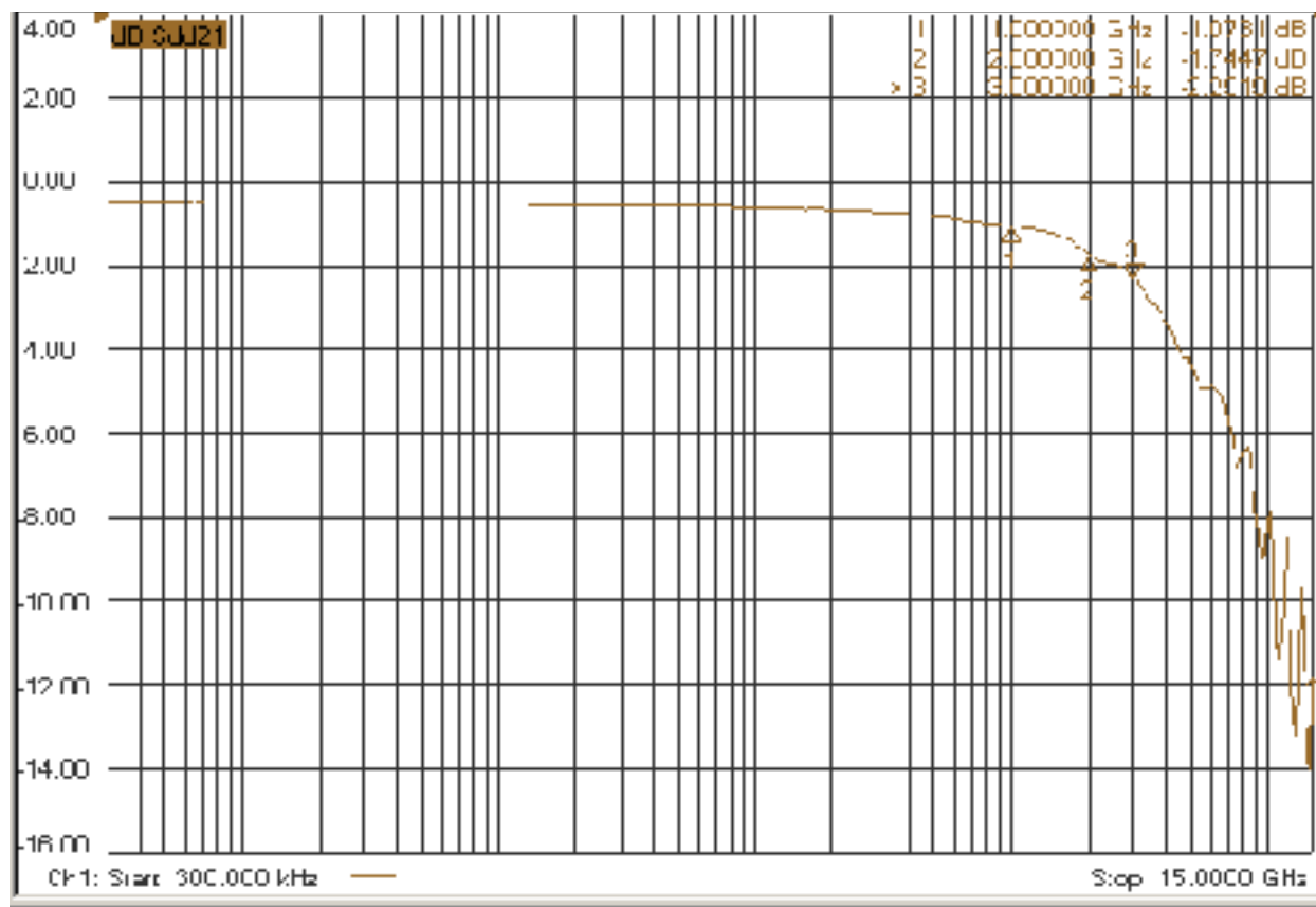
Insertion Loss
