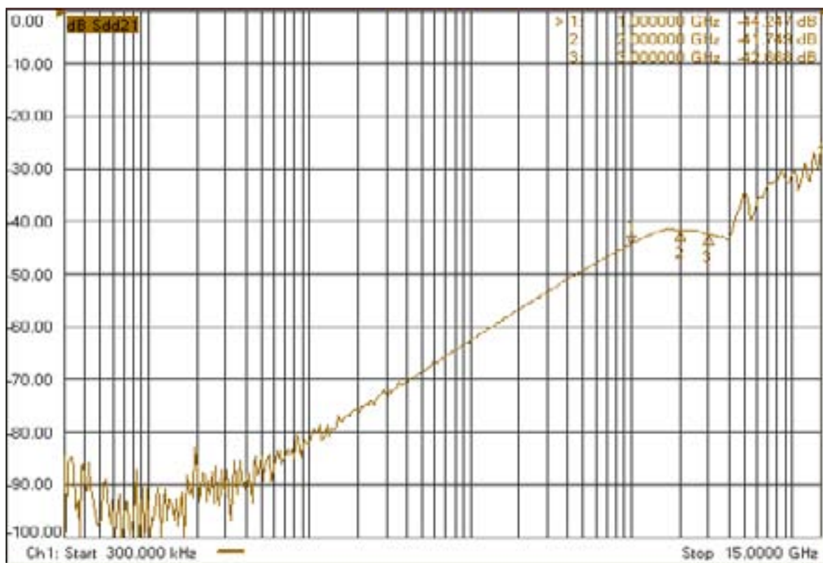
Crosstalk
