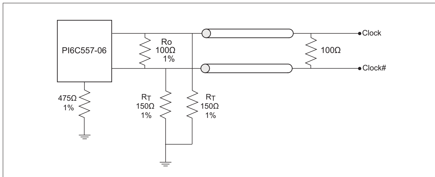
Test Load Board Termination for LVDS output
