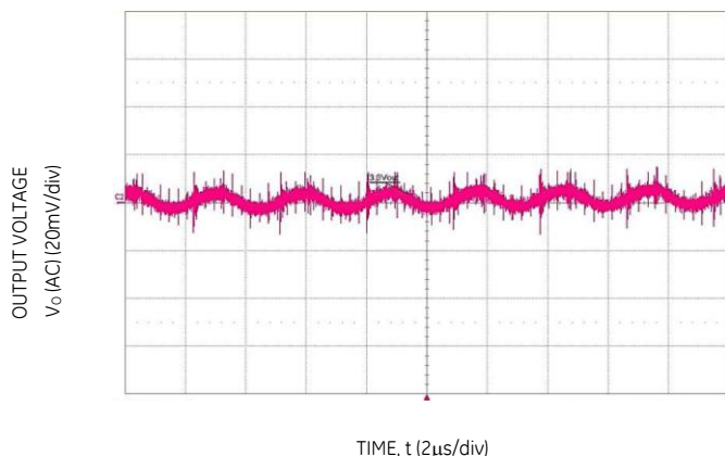
Fig 12: 3.3V Ripple
