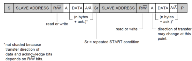
Fig 20: Typical I 2 C Read protocol
