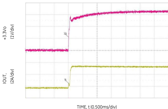
Fig 10: 3.3V Turn-On
