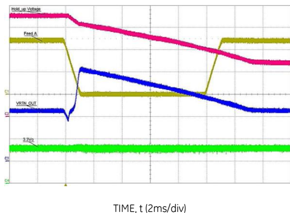
Fig 3: Hold-up Event vs 3.3Vout
