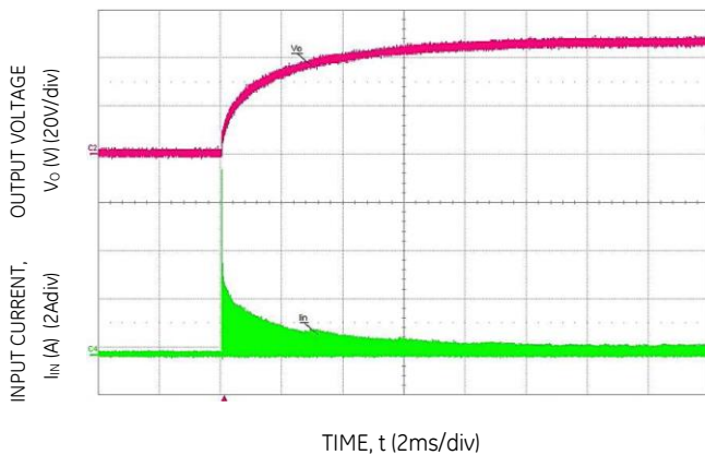
Figure 1. Inrush Current
