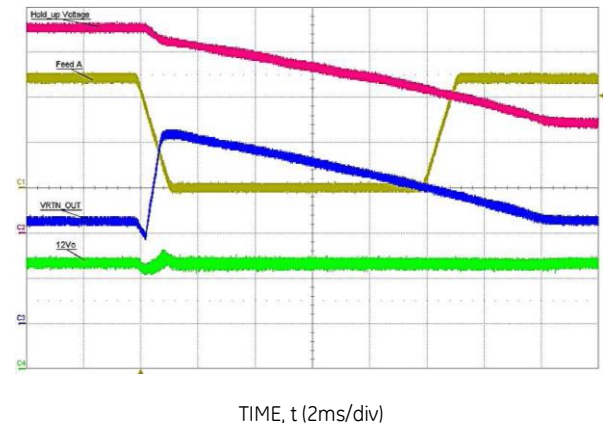
Fig 4: Hold-up Event vs 12.0Vout
