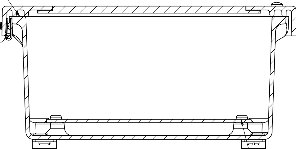
SECTION B-B
