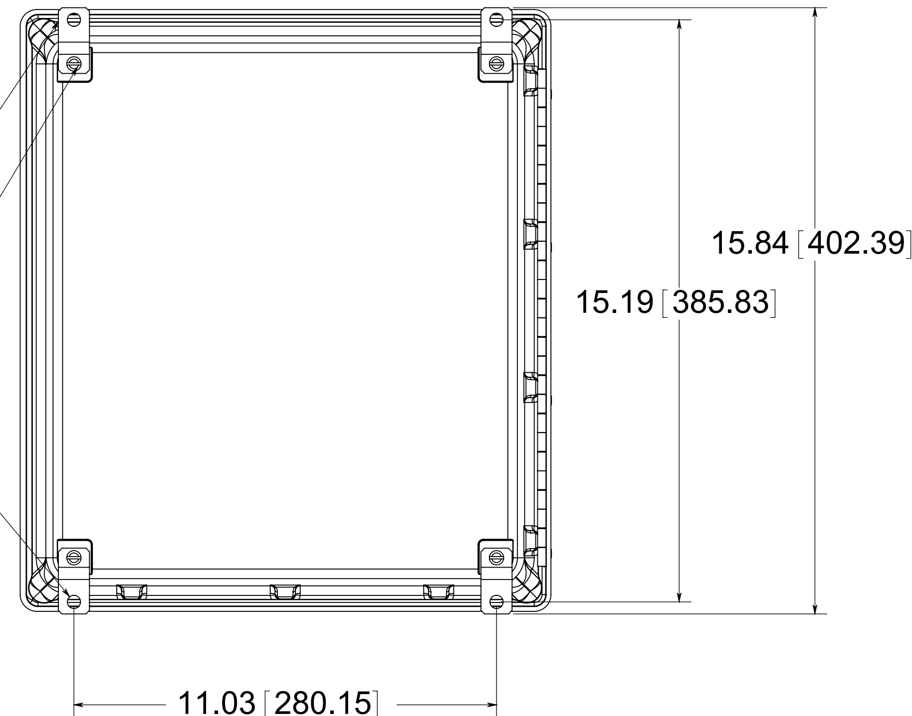
BACK VIEW
