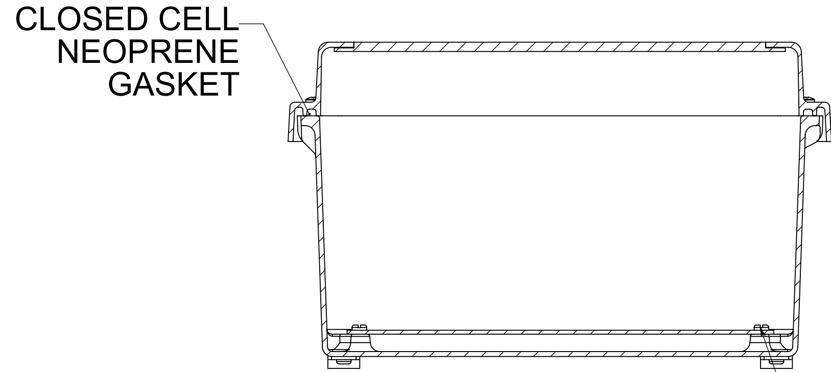
SECTION B-B
