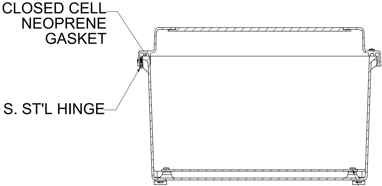
SECTION B-B
