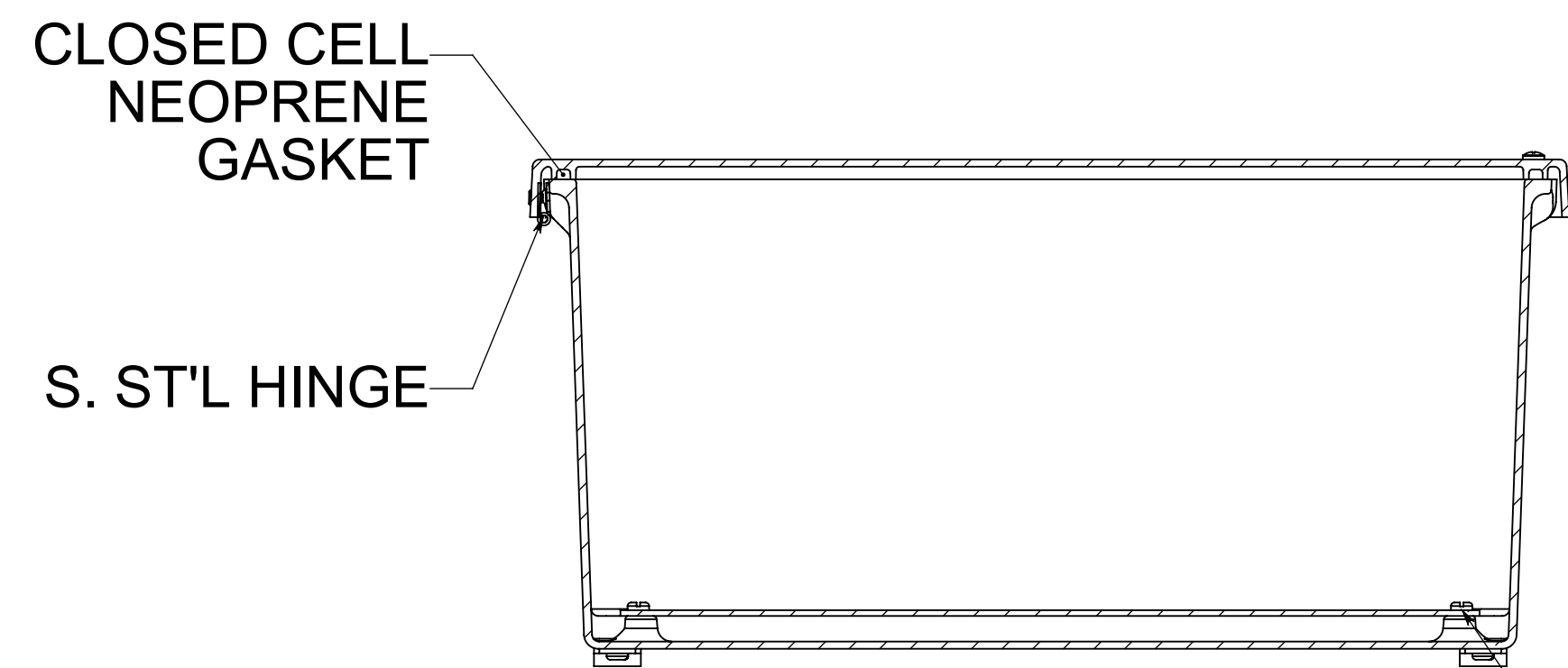
SECTION B-B
