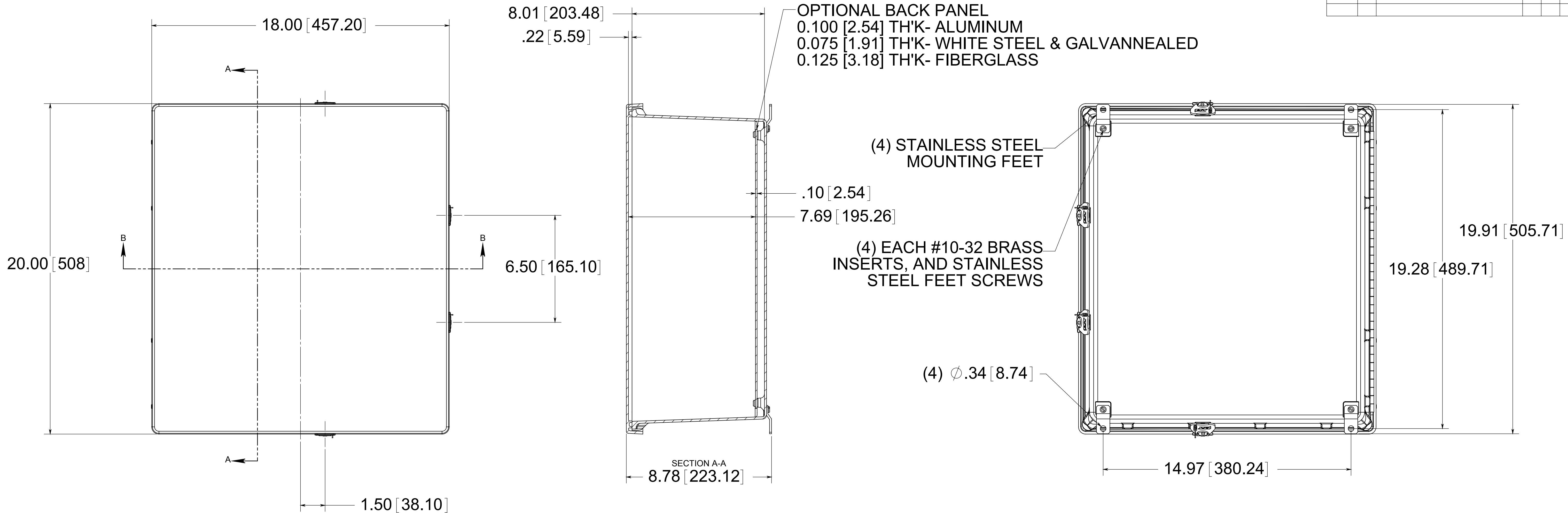
FRONT VIEW WITH COVER REMOVED AND BACK PANEL SHOWN
