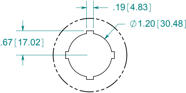
DETAIL C SCALE 2 : 3
