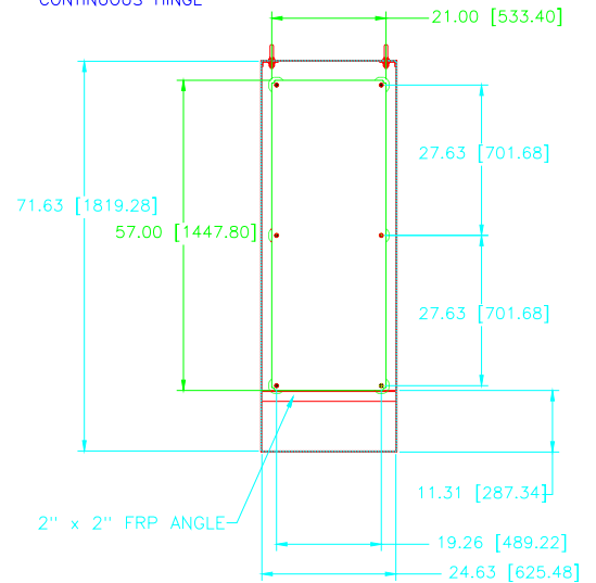
SECTION B-B
