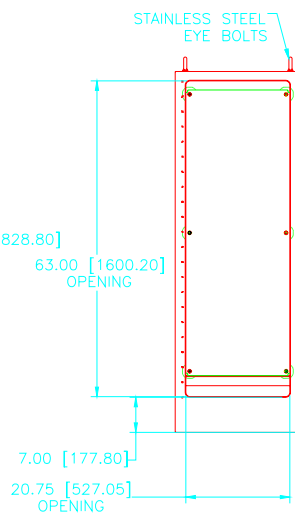
FRONT VIEW WITH DOOR & GASKET REMOVED
