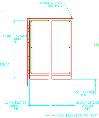
FRONT VIEW WITH DOORS REMOVED
