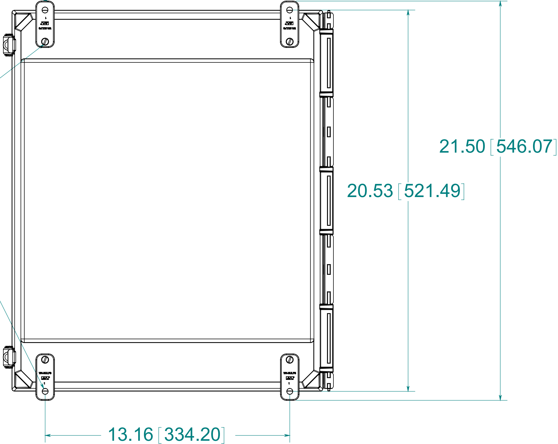
BACK VIEW
