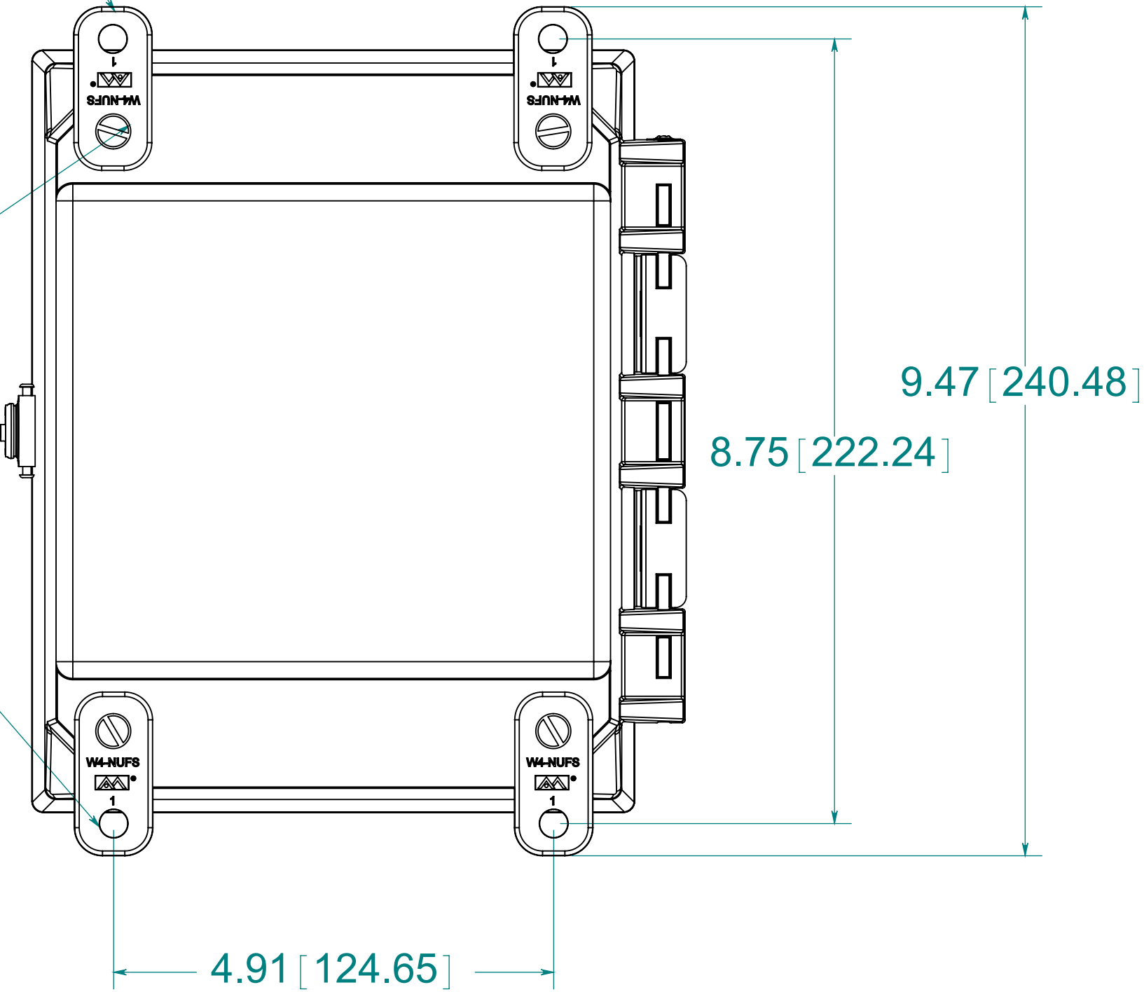
BACK VIEW
