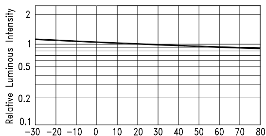
Fig.5 Luminous Intensity vs. Ambient Temperature
