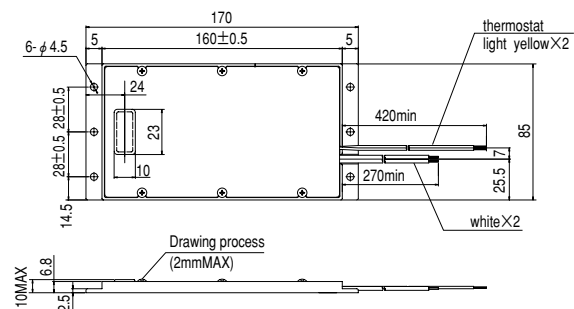
DV0P4282,DV0P4283
