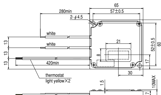
DV0P4280,DV0P4281
