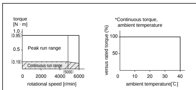
MAMA042□1□
