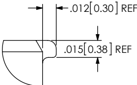
DETAIL 'J' SCALE 12:1
