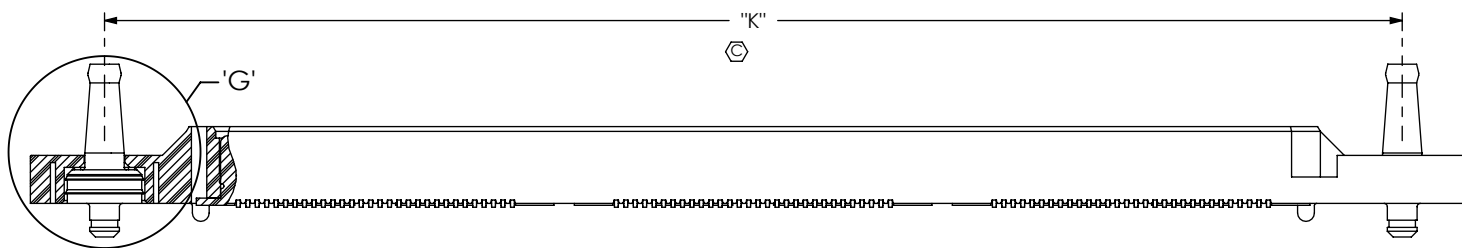
FIG 9 -RT1: RETENTION OPTION (QTH-060-01-X-D-DP-A-RT1 SHOWN) (FOR -01 LEAD STYLE ONLY) (NOT AVAILABLE WITH -LC OR -GP OPTIONS) (NOT AVAILABLE ON -080 & -100 POS) (DIFFERENT AS SHOWN, OTHERWISE SAME AS FIG 1)
