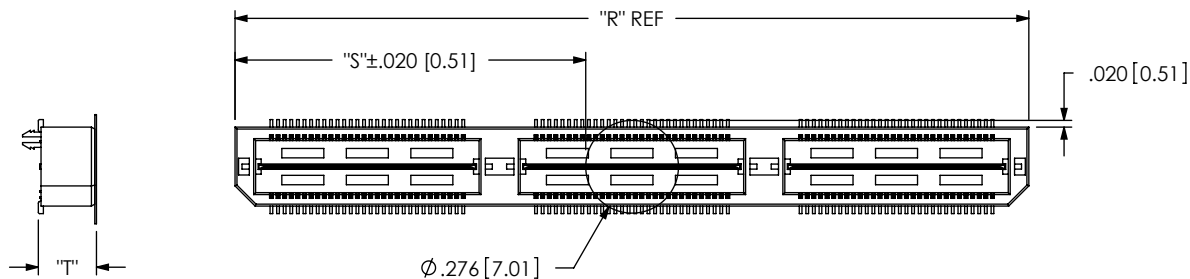
FIG 4 -K: POLYIMIDE FILM PAD OPTION (USE K-DOT-.276-.375-.005)
