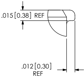
DETAIL 'F' SCALE 12:1
