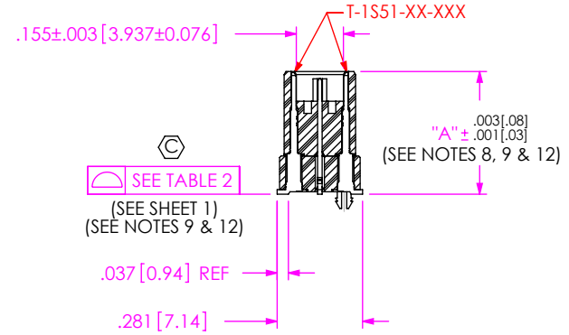
FIG 5 (QTS-075-03-XXX-D-LC SHOWN) (DIFFERENT AS SHOWN, OTHERWISE SAME AS FIG 1)
