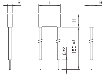
Insulated flexible leads 0.5mm 2
