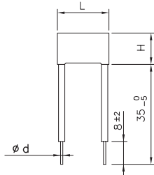
Insulated rigid leads
