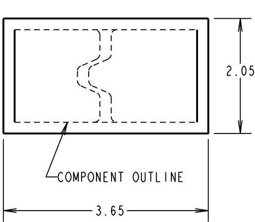
RECOMMENDED PAD LAYOUT
