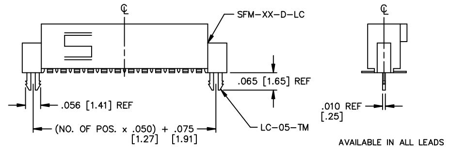
FIGURE 6 -LC OPTION DIFFERENT AS SHOWN, OTHERWISE SAME AS FIGURE 1
