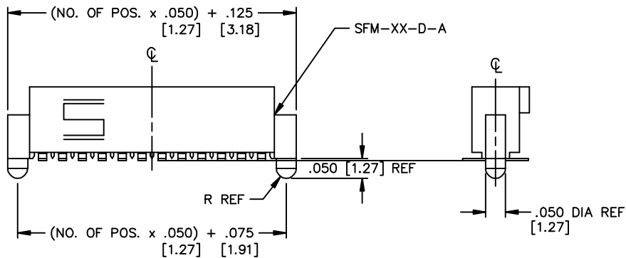
FIGURE 5 -A OPTION DIFFERENT AS SHOWN, OTHERWISE SAME AS FIGURE 1
