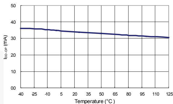
Figure 7. Operating Supply Current ( I_{DD-OP} ) vs. Temperature
