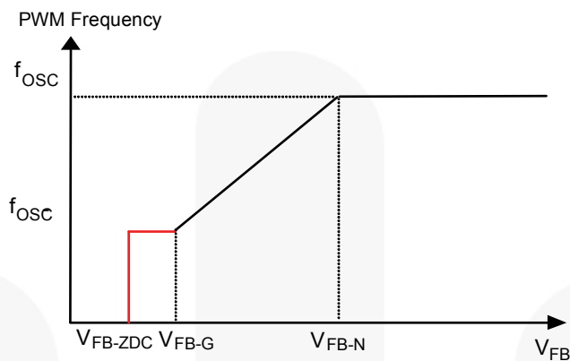
Figure 5. PWM Frequency
