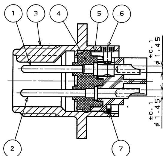
SECT. A-A
