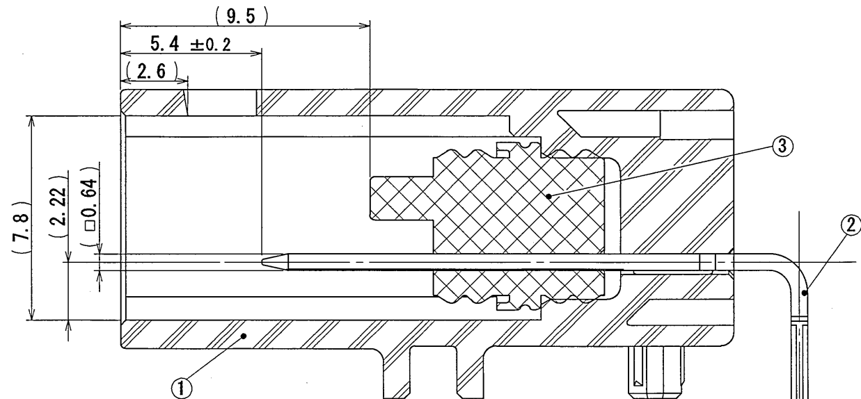
SECT. X-X (SCALE 5:1)
