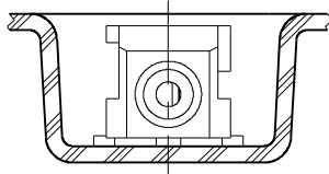
SECT. B-B (SCALE 5:1)
