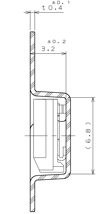
SECT. C-C (SCALE 5:1)
