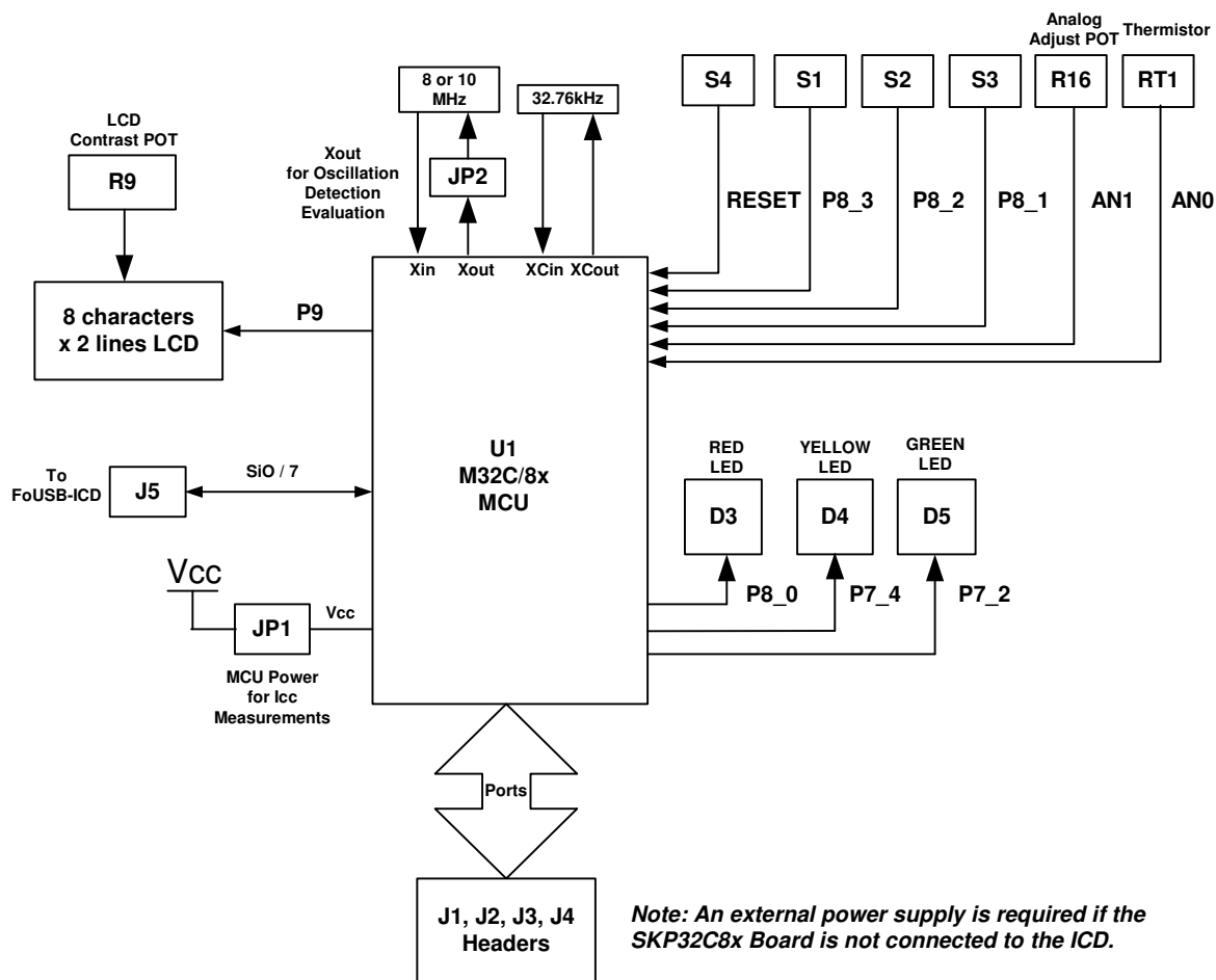
Figure 5-2. SKP32C8x Block Diagram
