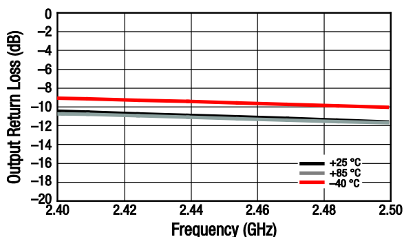
Figure 7. Small Signal Output Return Loss (IS22) vs Frequency and Temperature, Narrow Band
