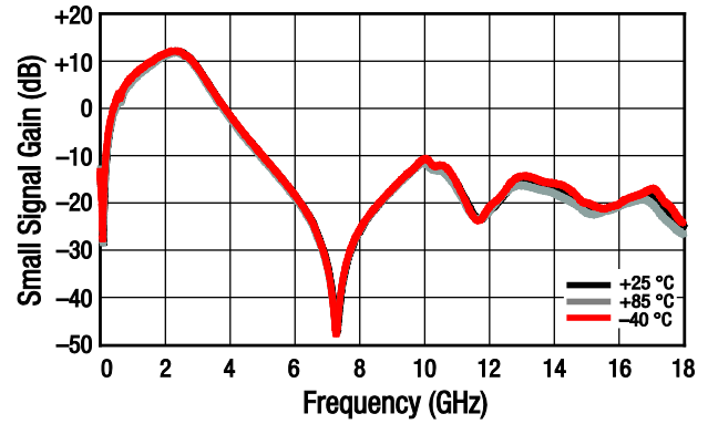
Figure 21. Small Signal Gain (IS21I) vs Frequency and Temperature, Wide Band
