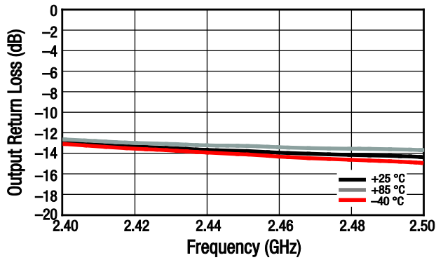
Figure 20. Small Signal Output Return Loss (IS22I) vs Frequency and Temperature, Narrow Band
