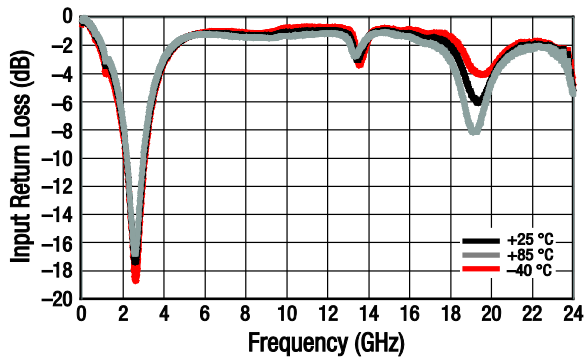
Figure 9. Small Signal Input Return Loss (S11) vs Frequency and Temperature, Wide Band
