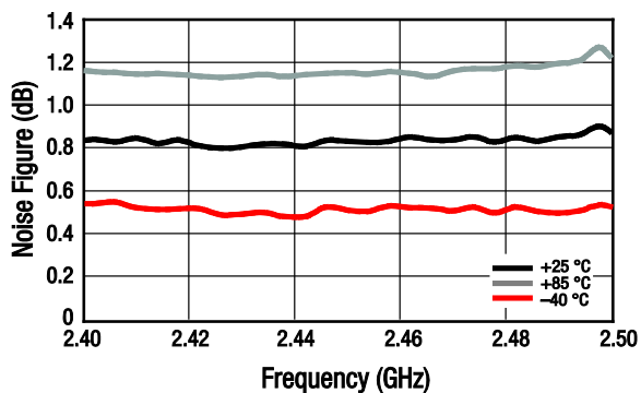
Figure 3. Noise Figure vs Frequency and Temperature, Narrow Band (Includes EVB Insertion Losses)
