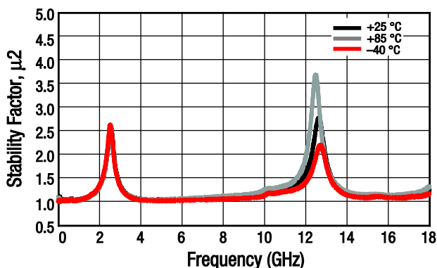
Figure 26. Stability Factor ( \mu_2 ) vs Frequency and Temperature, Wide Band
