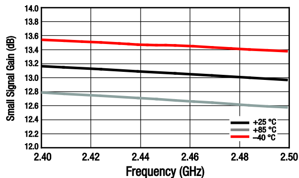
Figure 4. Small Signal Gain (IS21) vs Frequency and Temperature, Narrow Band
