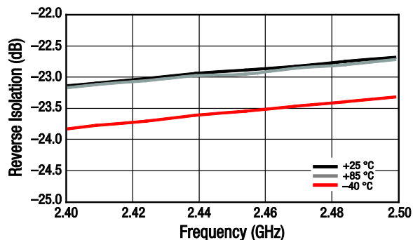
Figure 6. Small Signal Reverse Isolation (IS12) vs Frequency and Temperature, Narrow Band
