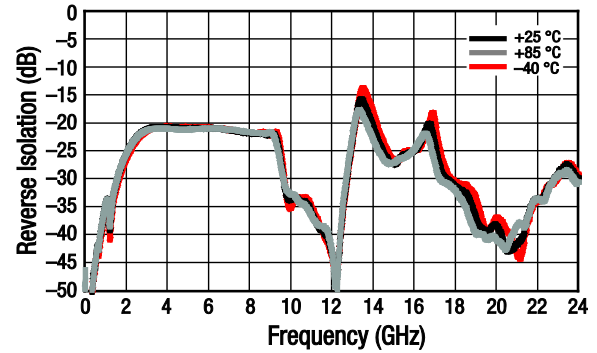
Figure 10. Small Signal Reverse Isolation (S12) vs Frequency and Temperature, Wide Band
