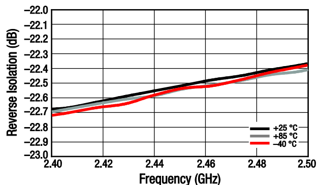
Figure 19. Small Signal Reverse Isolation (IS12) vs Frequency and Temperature, Narrow Band
