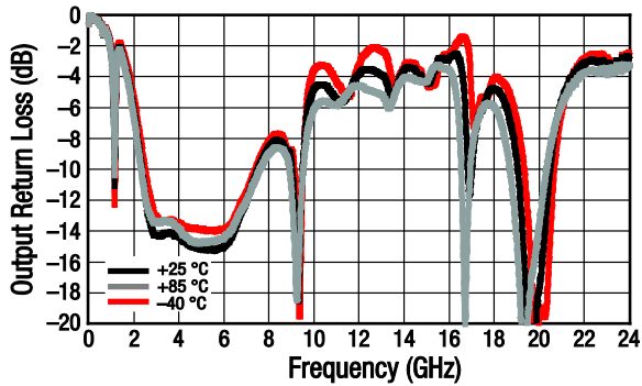
Figure 11. Small Signal Output Return Loss (S22) vs Frequency and Temperature, Wide Band
