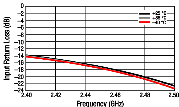
Figure 18. Small Signal Input Return Loss (IS11) vs Frequency and Temperature, Narrow Band
