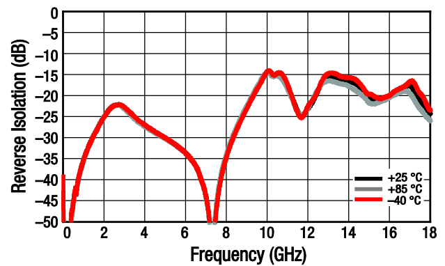
Figure 23. Small Signal Reverse Isolation (I S12 I) vs Frequency and Temperature, Wide Band
