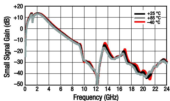
Figure 8. Small Signal Gain (IS21) vs Frequency and Temperature, Wide Band
