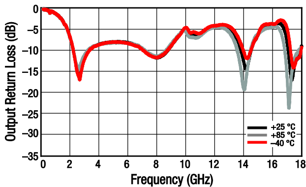
Figure 24. Small Signal Output Return Loss (I S22 I) vs Frequency and Temperature, Wide Band
