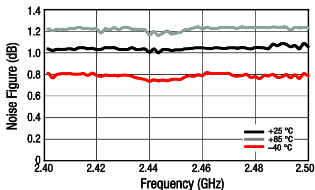
Figure 16. Noise Figure vs Frequency and Temperature, Narrow Band (Includes EVB Insertion Losses)
