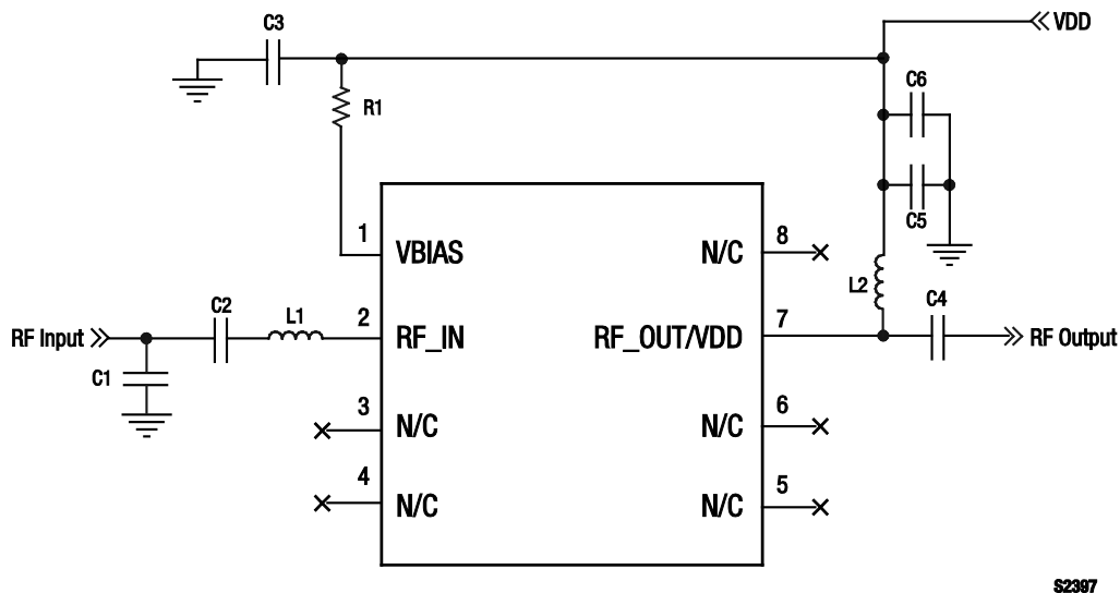
Figure 28. SKY67014-396LF Evaluation Board Schematic
