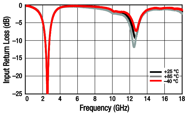
Figure 22. Small Signal Input Return Loss (I S11 I) vs Frequency and Temperature, Wide Band
