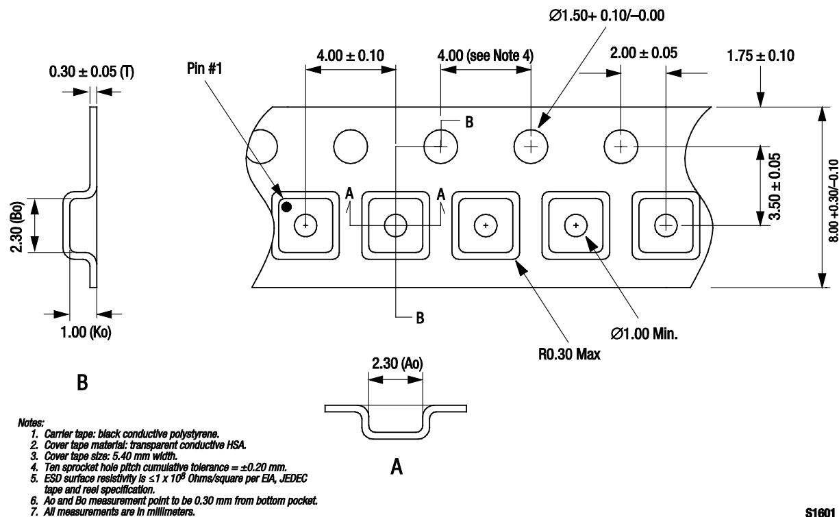
Figure 32. SKY67014-396LF Tape and Reel Dimensions
