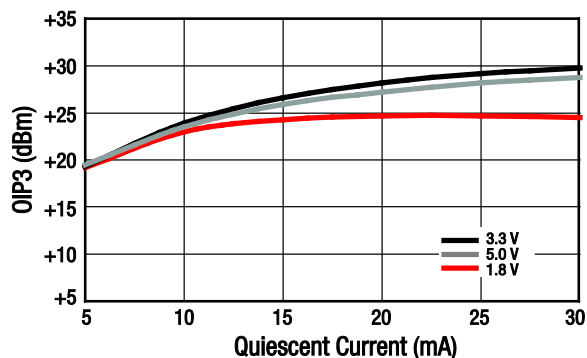
Figure 15. OIP3 vs Quiescent Current and Voltage
