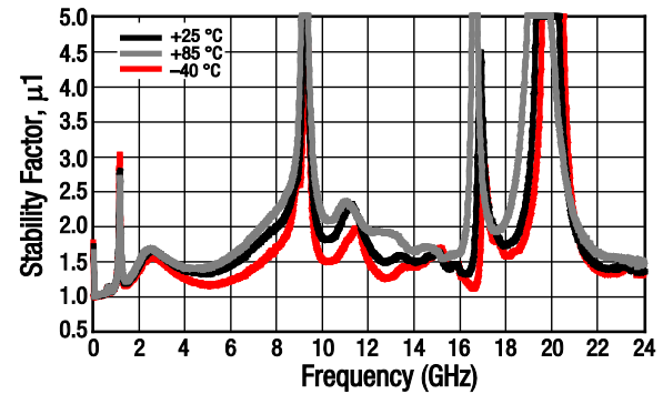
Figure 12. Stability Factor ( \mu_1 ) vs Frequency and Temperature, Wide Band
