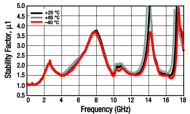
Figure 25. Stability Factor ( \mu_1 ) vs Frequency and Temperature, Wide Band
