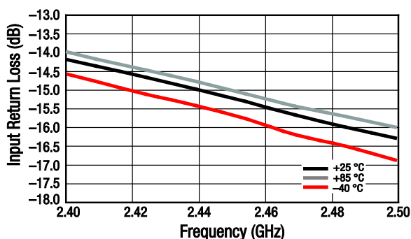
Figure 5. Small Signal Input Return Loss (IS11) vs Frequency and Temperature, Narrow Band
