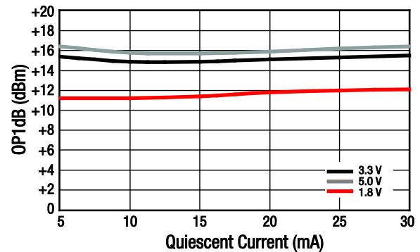
Figure 14. OP1dB vs Quiescent Current and Voltage
