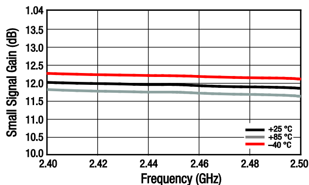
Figure 17. Small Signal Gain (IS21) vs Frequency and Temperature, Narrow Band
