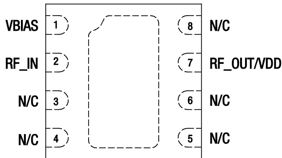
Figure 2. SKY67014-396LF Pinout – 8-Pin DFN (Top View)
