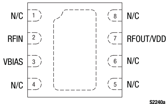
Figure 2. SKY67151-396LF Pinout – 8-Pin DFN (Top View)
