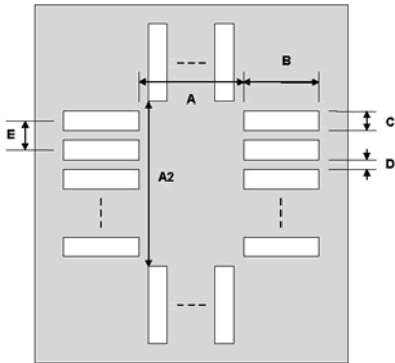
Top View (SMT Footprint)
