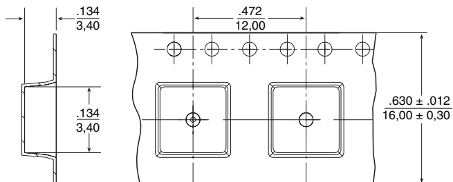
TAPE & REEL LAYOUT
