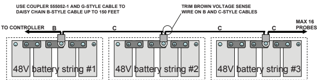
Temperature Measurement
