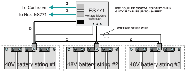
Temperature/Voltage Measurement
