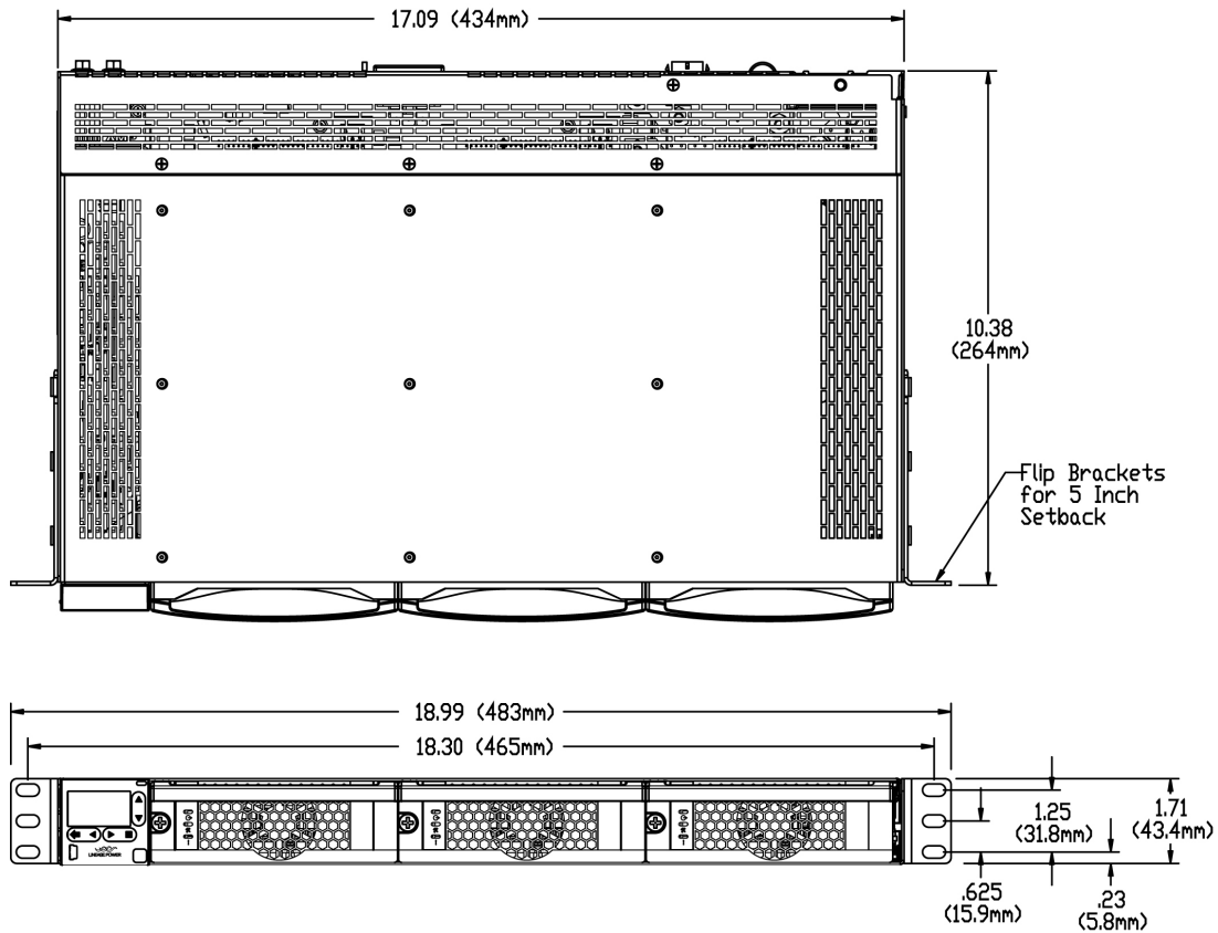
Shelf Line Drawing - J2007003
