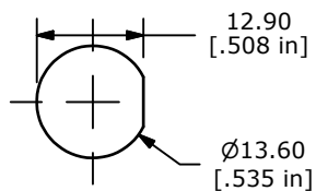
PANEL MOUNTING
