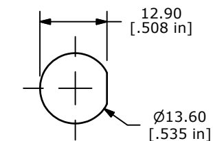
PANEL MOUNTING
