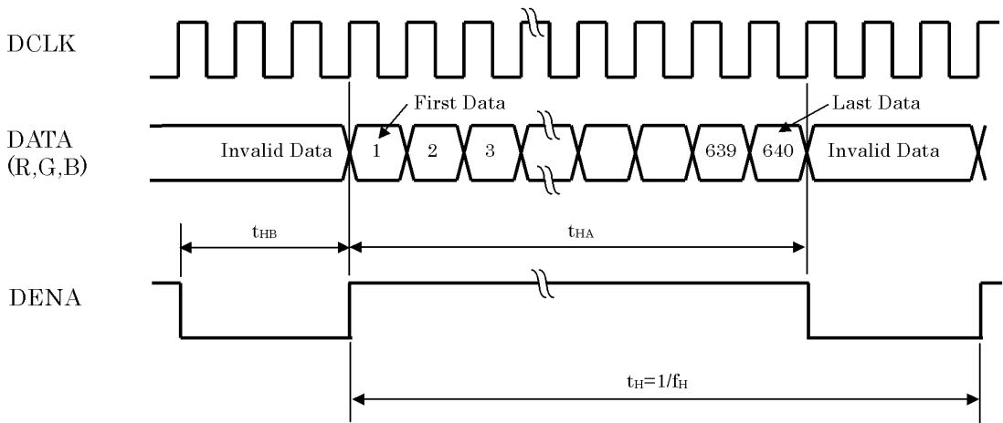
b. Horizontal Timing Chart
