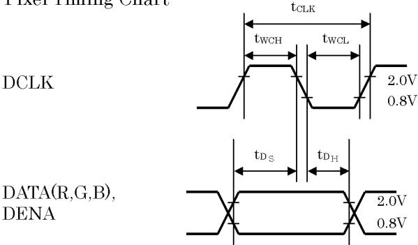
a. Pixel Timing Chart
