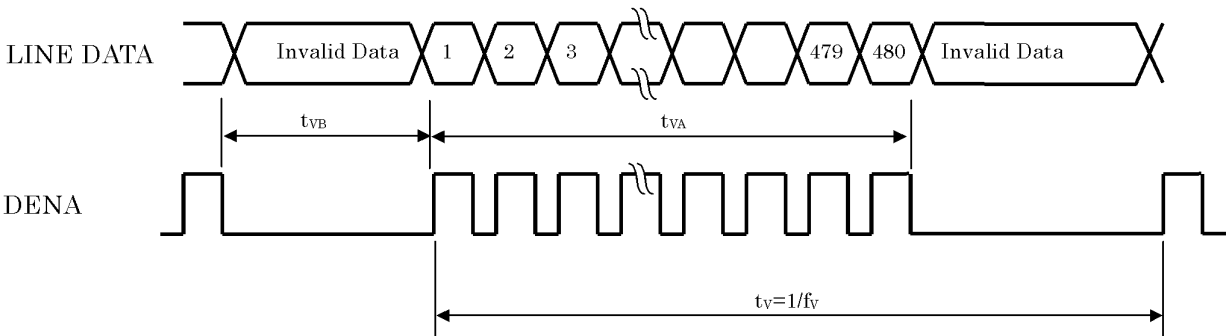
c. Vertical Timing Chart
