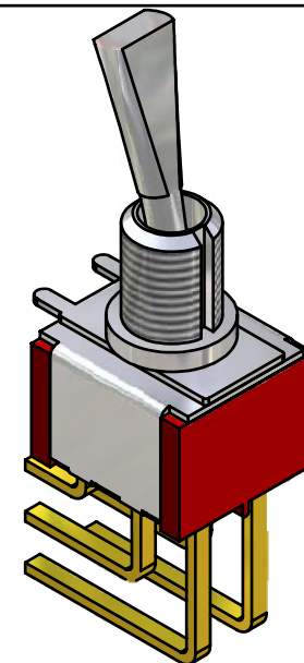
ISOMETRIC
