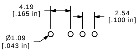
PC MOUNTING
