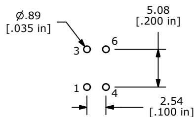
PC MOUNTING
