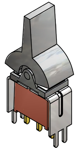
ISOMETRIC
