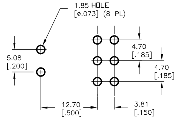
RECOMMENDED PCB LAYOUT SCALE 2:1
