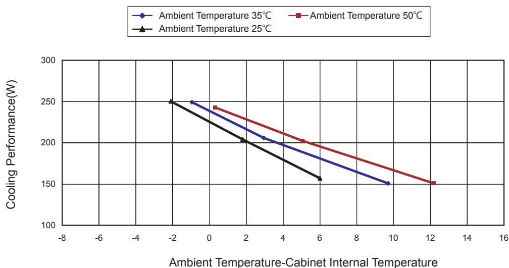
Cooling Performance VS Temperature Difference
