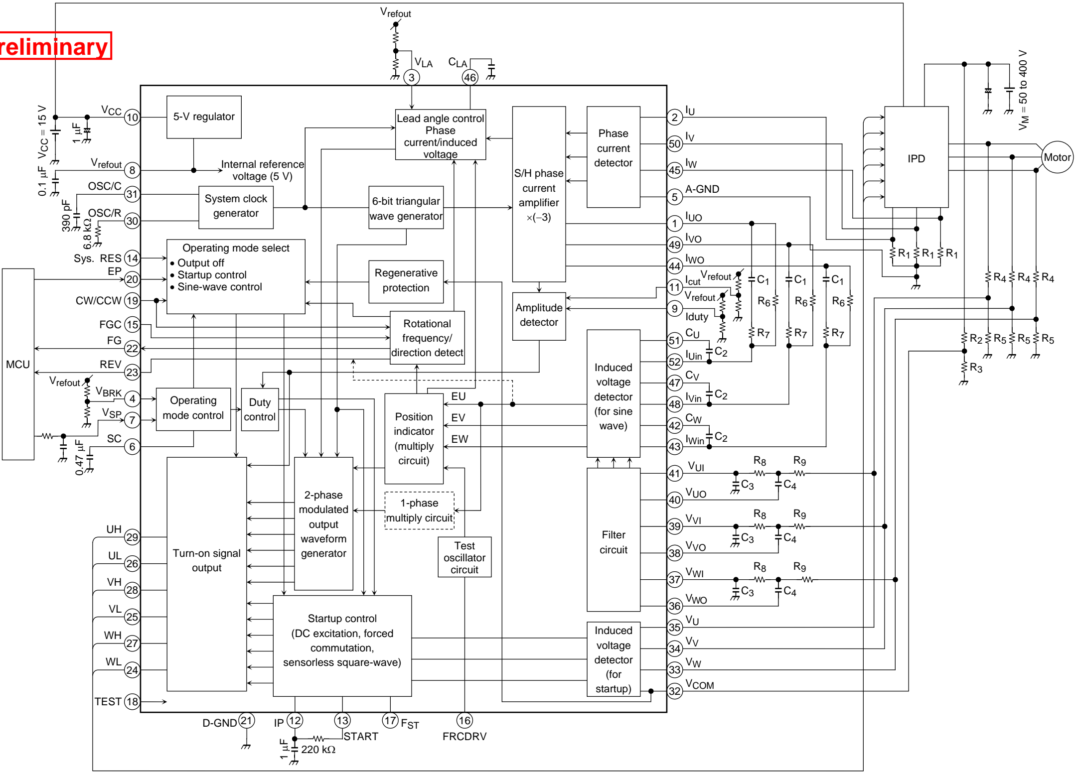
Block Diagram
